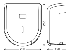
CLEANLINE JUMBO 200
