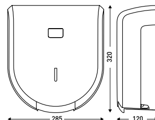
CLEANLINE JUMBO 400
