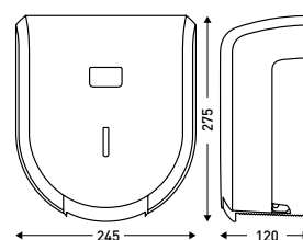
CLEANLINE JUMBO 400
